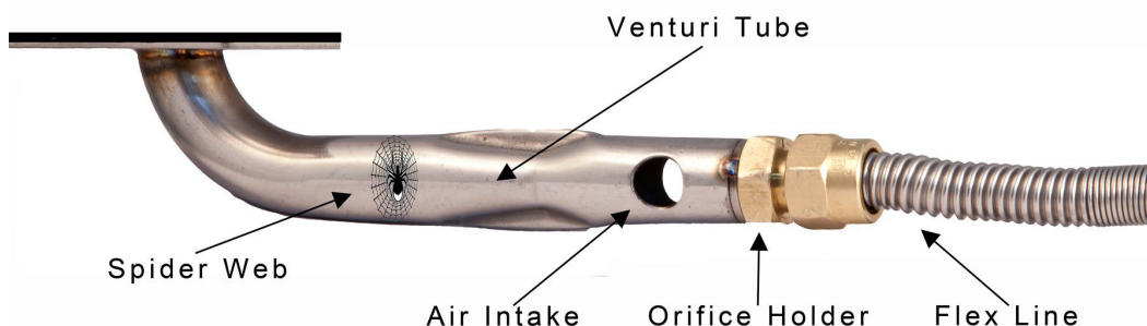
SIDE VIEW OF VENTURI ASSEMBLY
